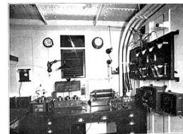
Marconi Company receiving equipment for a 5 kilowatt ocean liner station (in the picture, the wireless radio room of Titanic 's sister ship, the Olympic )
