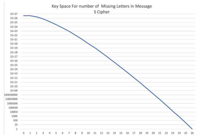
Fig. 1. Key Space vs. Unseen Characters
